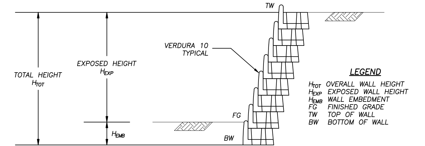
TYPICAL CROSS SECTION DETAIL
