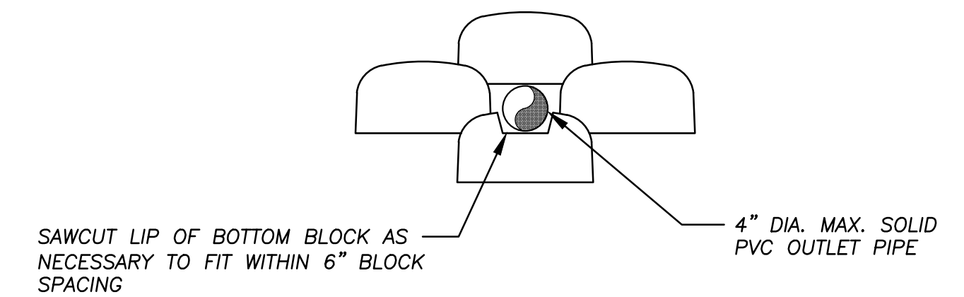
TYPICAL PENETRATION DETAIL
