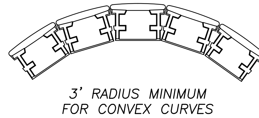
RADIUS FOR CONVEX CURVES DETAIL
