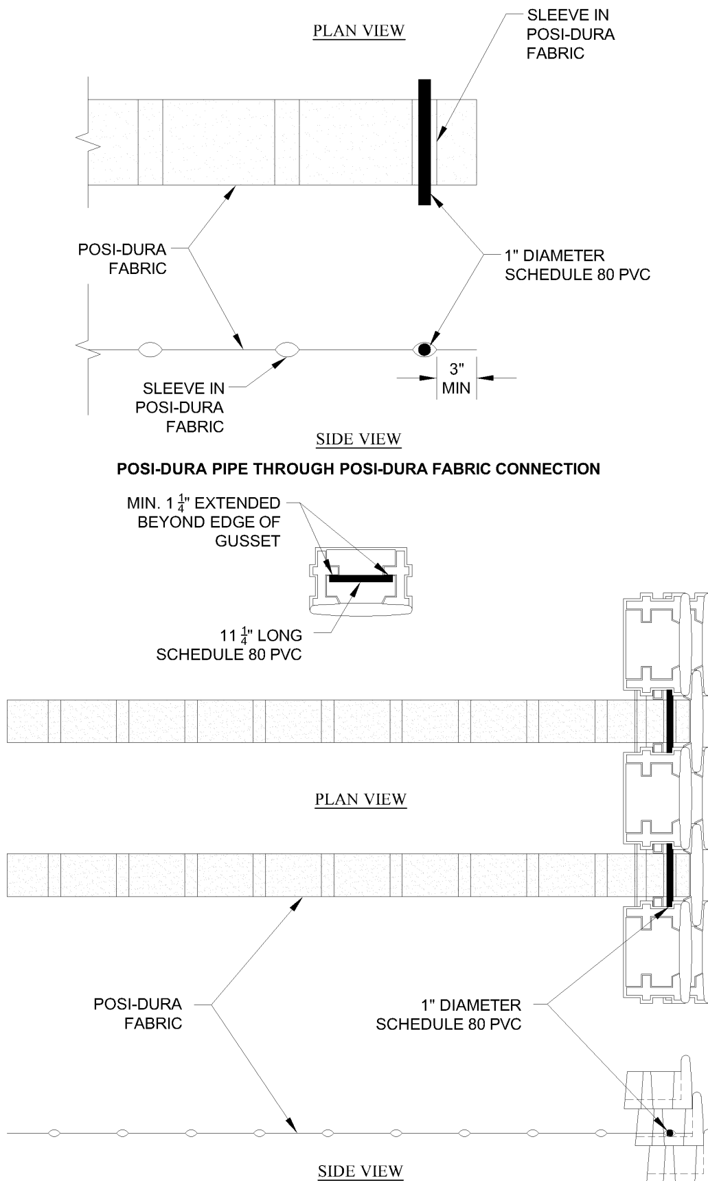
FIGURE 4 - POSI-DURA REINFORCEMENT CONNECTION
