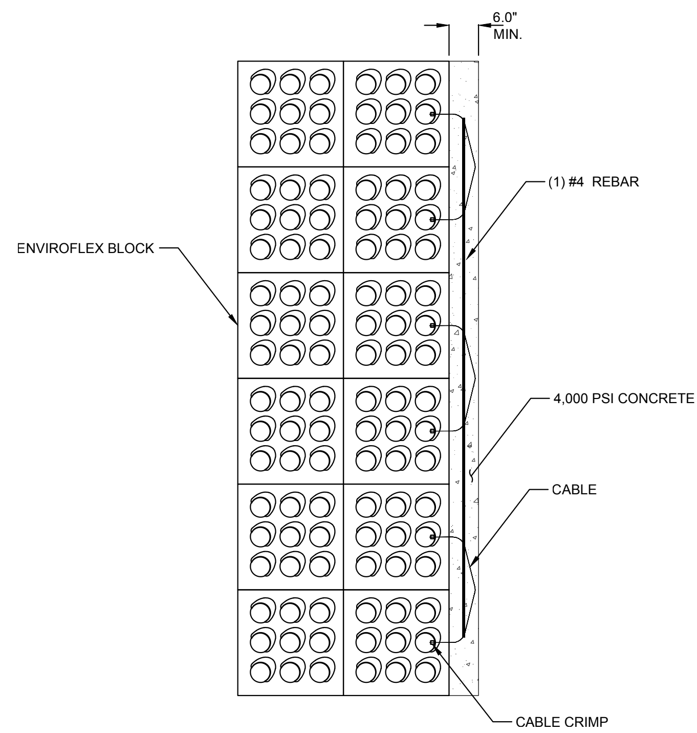
SQUARE BLOCK TO CONCRETE EDGE DETAIL
