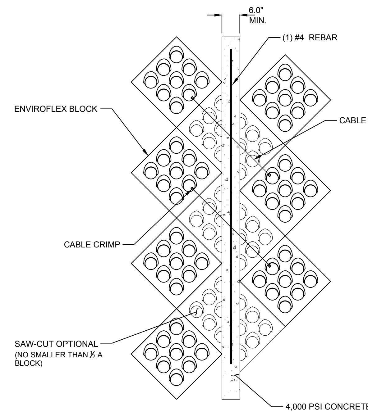
DIAGONAL BLOCK TO DIAGONAL BLOCK THRU GRADE BREAK DETAIL
