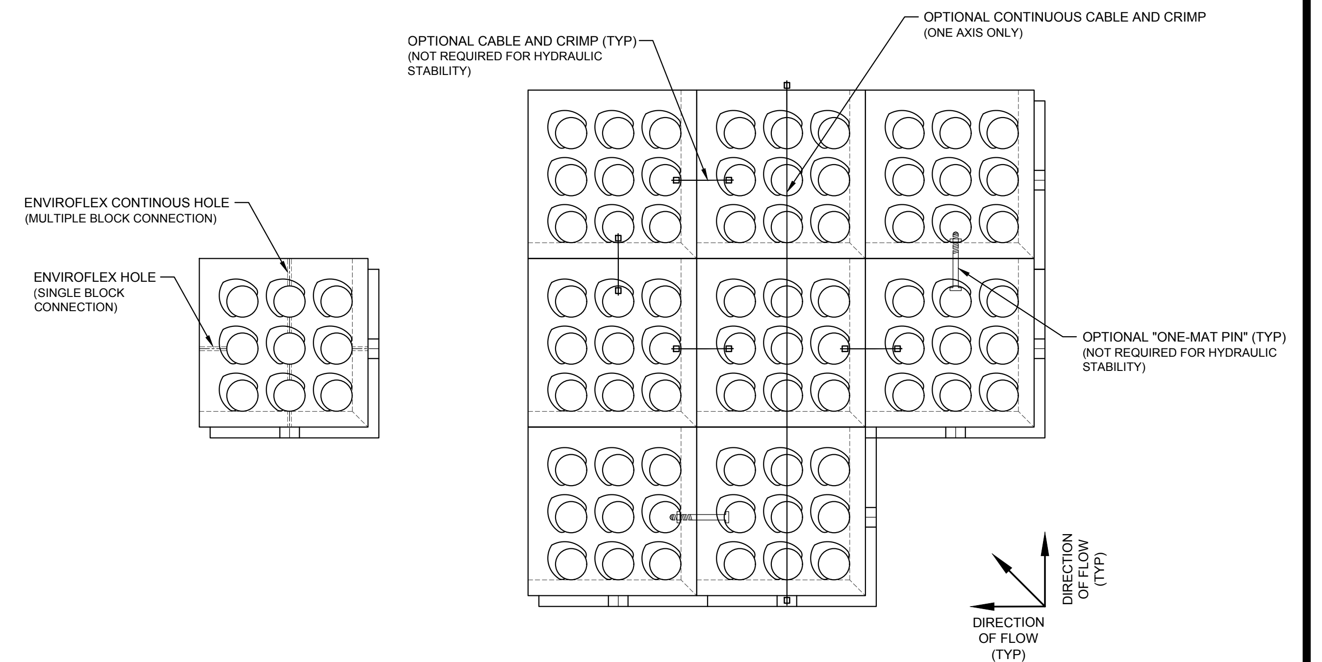
ENVIROFLEX® BLOCK TO BLOCK CONNECTION OPTIONS
