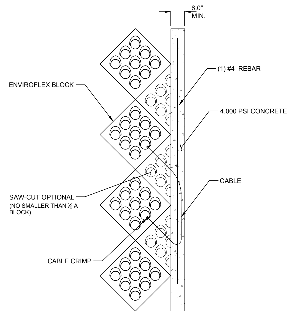
DIAGONAL BLOCK TO CONCRETE EDGE DETAIL
