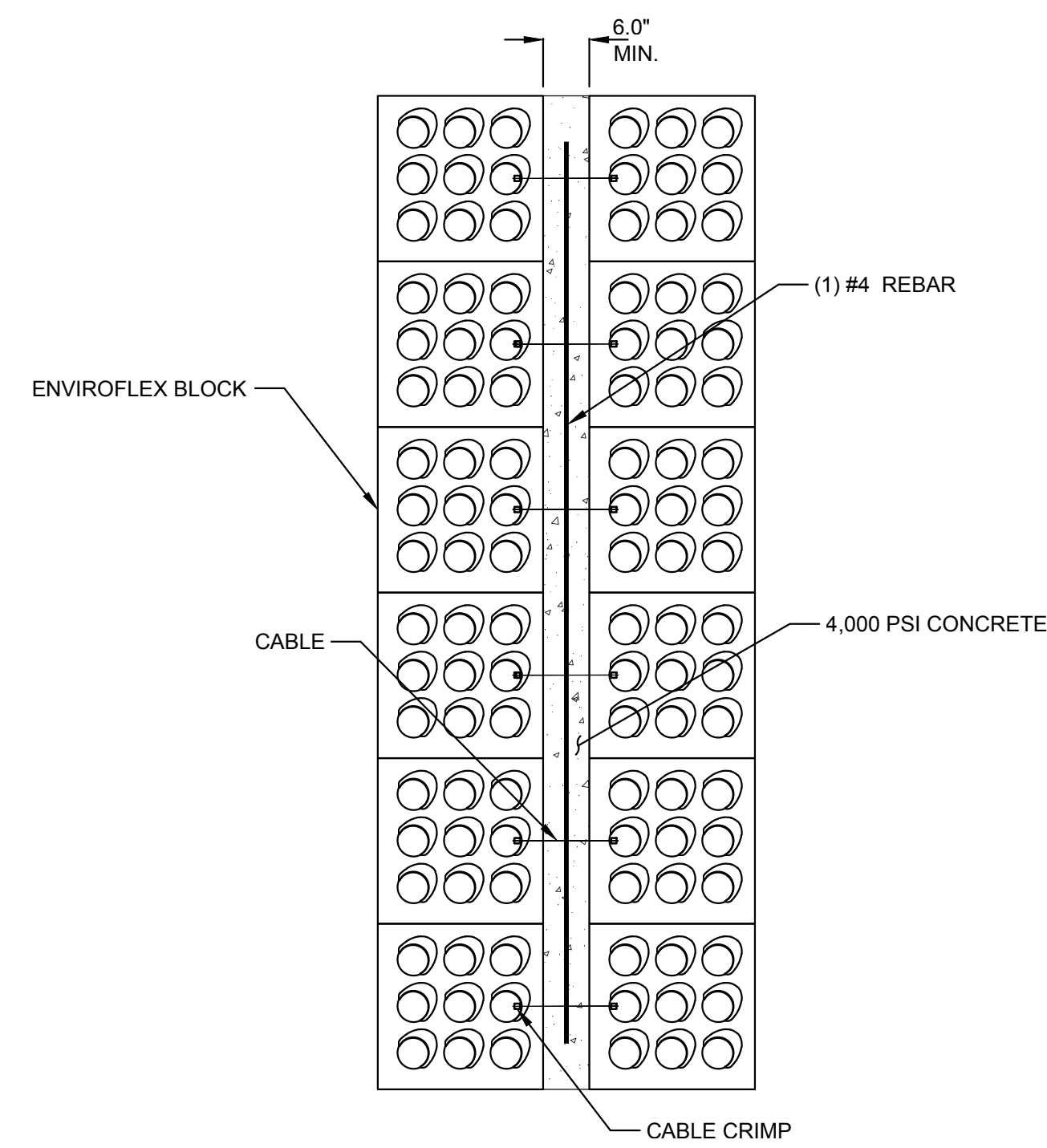
SQUARE BLOCK TO SQUARE BLOCK THRU GRADE BREAK DETAIL
