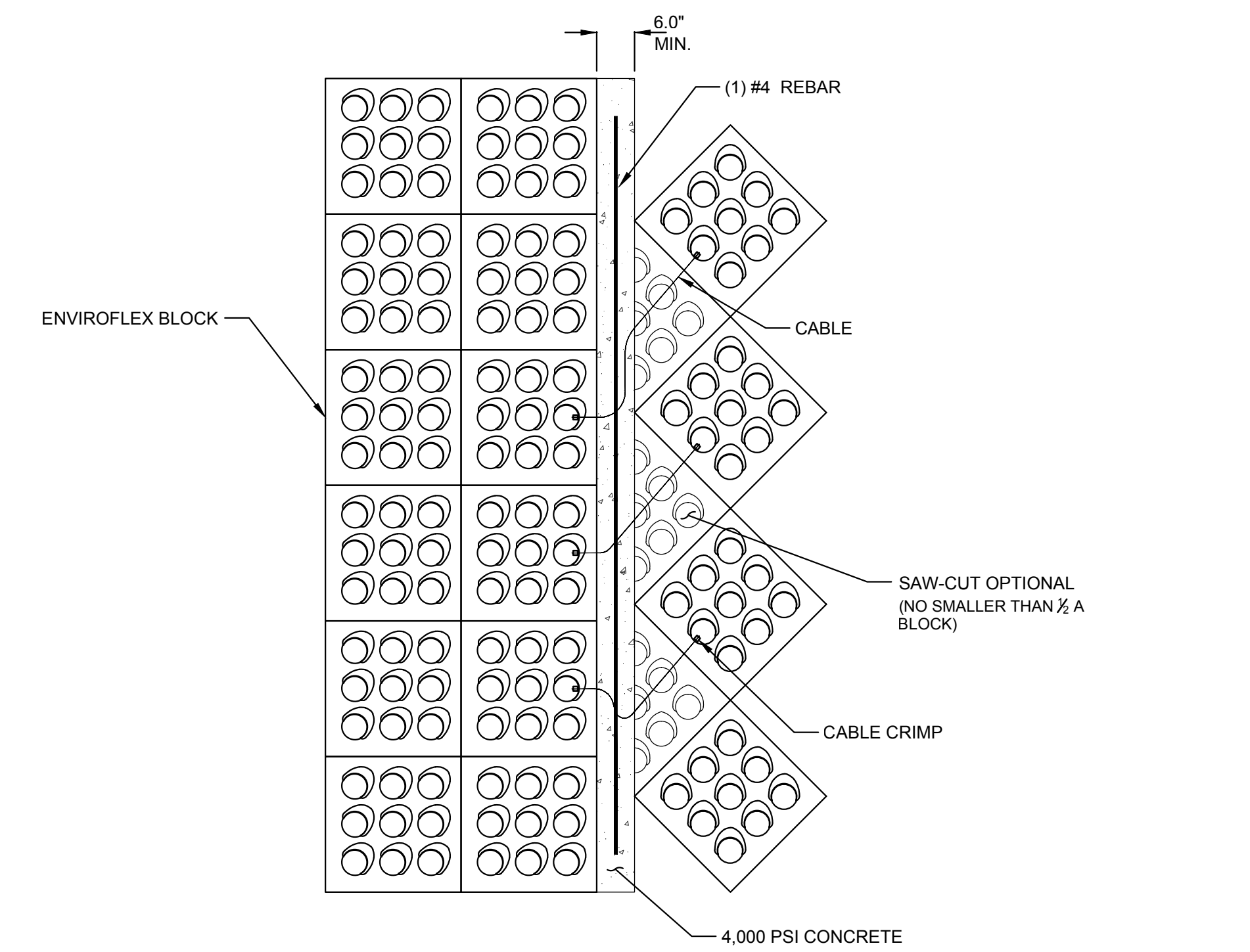
SQUARE BLOCK TO DIAGONAL BLOCK THRU GRADE BREAK DETAIL
