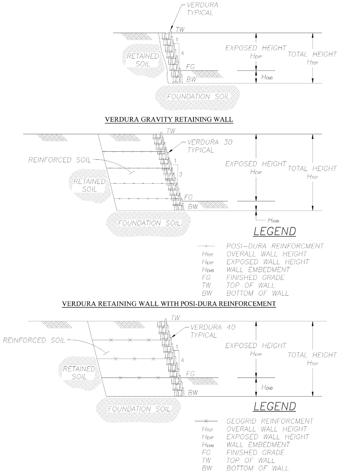
FIGURE 6 - TYPICAL WALL SECTIONS
