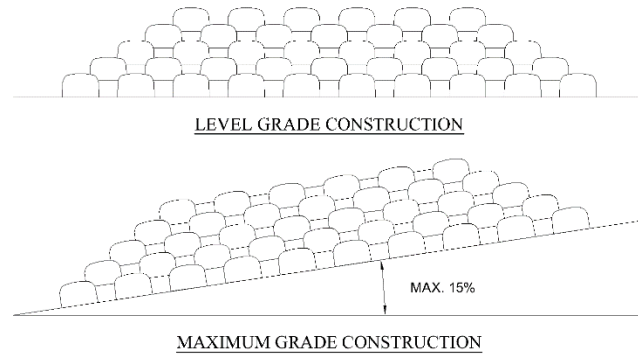
FIGURE 3 - TYPICAL GRADE CONSTRUCTION
