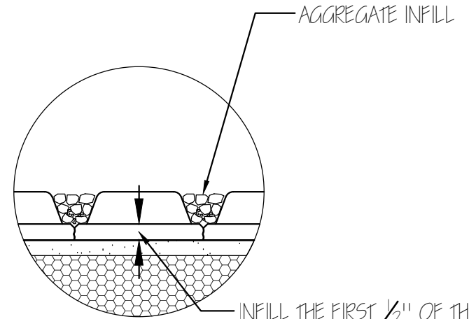
INFILL DETAIL
